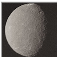
Umbriel Uranus,
